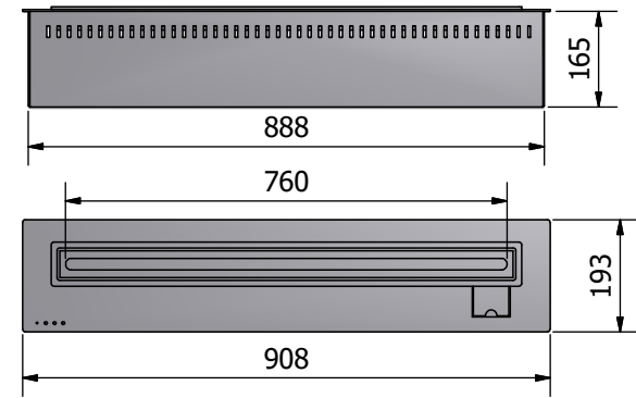
Automatic burner ProFire L908
